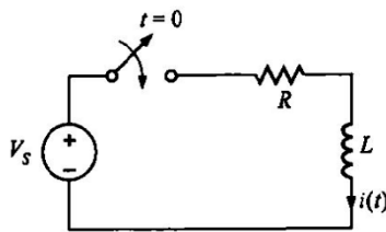
Figura 1. Circuito resistor-inductor (RL).
